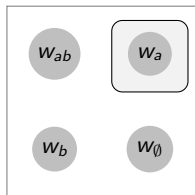
(b) \models (a \vee_{1/2/3} b)
