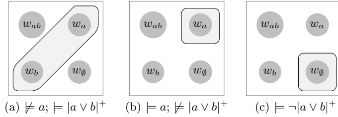
Fig. 3. Illustrations of supporting states in BiUS
